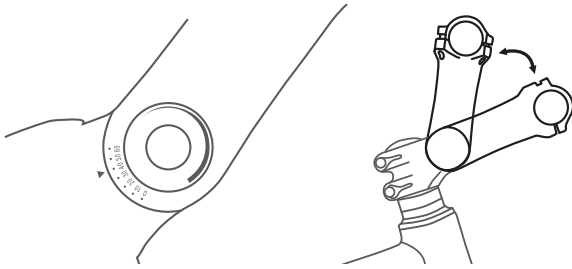
Figure 59: Different versions of angle-adjustable stems
