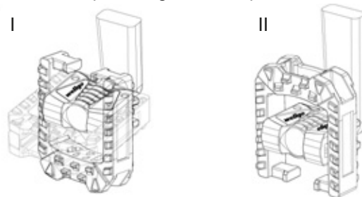
Figure 85: Folding the pedal up (I) or down (II)
