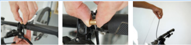
Figure 151: Unfastening the remote control
