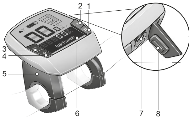
Figure 31: BOSCH Intuvia on-board computer layout
