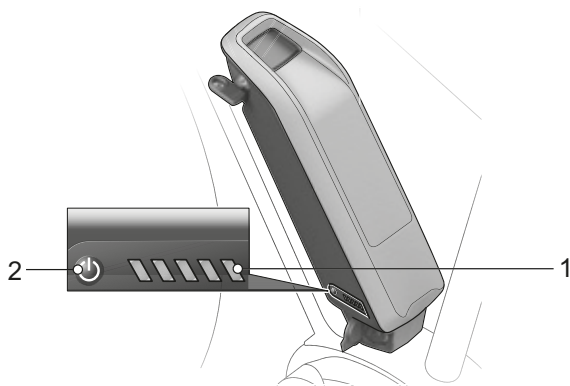
Figure 36: Position of battery level indicator on seat tube battery
