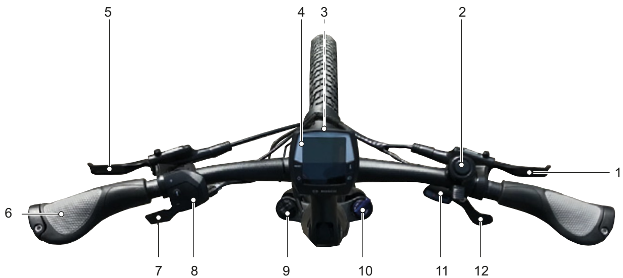
Figure 30: Detailed view of handlebars with BOSCH Intuvia on-board computer, example
