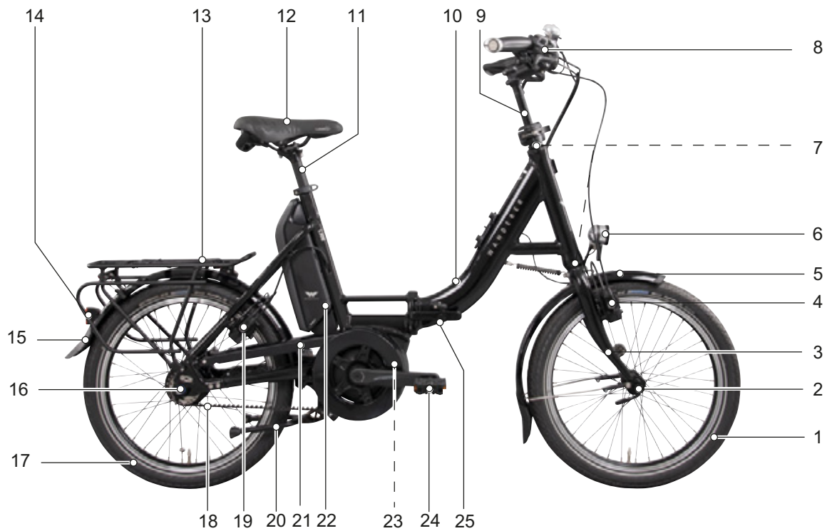
Figure 2: Pedelec viewed from the right, example
