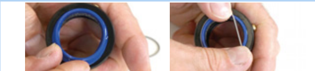
Figure 126: inserting and fastening the wiper
