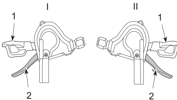
Figure 83: Down shifter (1) and up shifter (2) on the left (I) and right (II) gear shift
